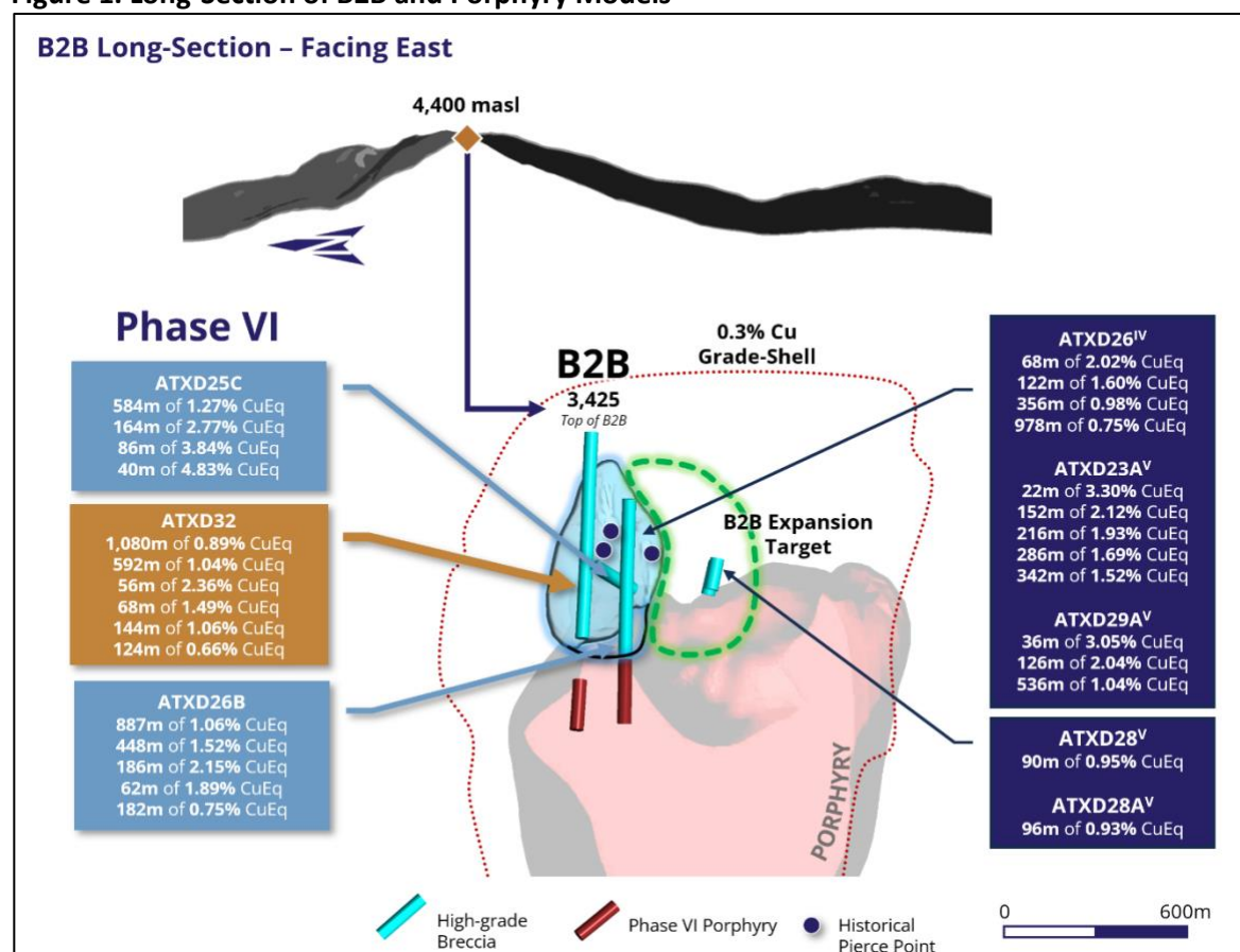
Figure 1. Long-Section of B2B and Porphyry Models iv
