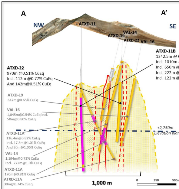
FIGURE 2A: VALERIANO PROJECT ATXD-11B CROSS SECTION
